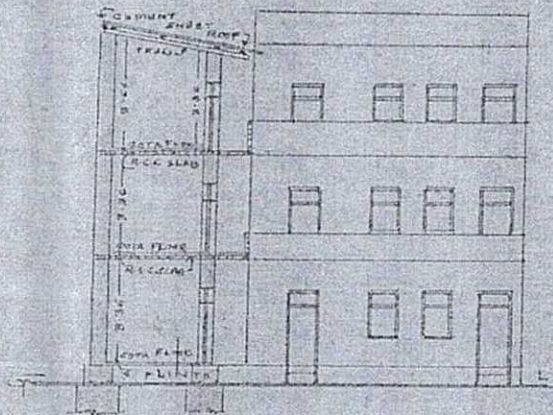
SECTIONAL ELEVATION ON A-B.
